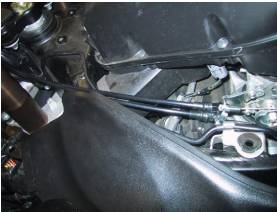
Cables mounted to the throttle body and routed along the frame.
